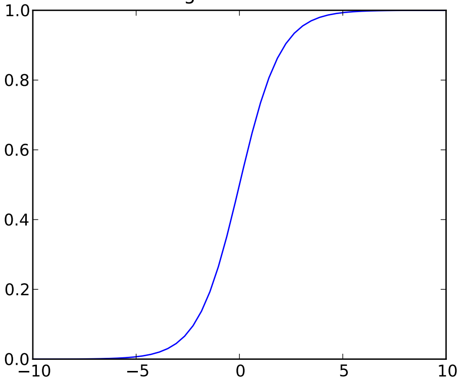
Logistic function
